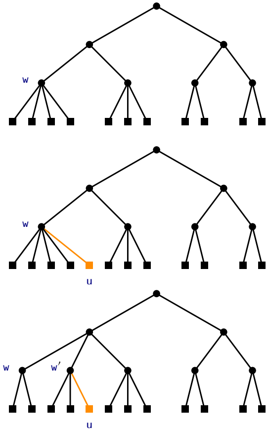
Figure 9.2: Adding a leaf to a 2-4 Tree. This process stops after one split because w .parent has a degree of less than 4 before the addition.
