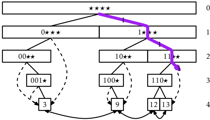
Figure 13.6: Since there is no node labelled 111* , the search path for 14 (1110) ends at the node labelled 11** .
