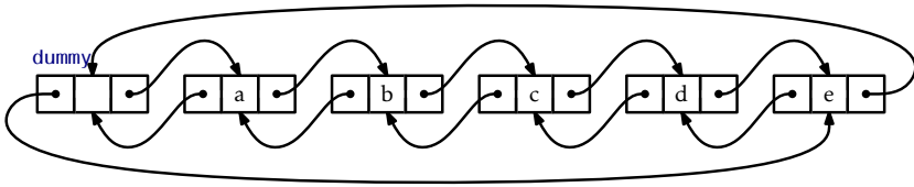
Figure 3.2: A DLL list containing a,b,c,d,e.
